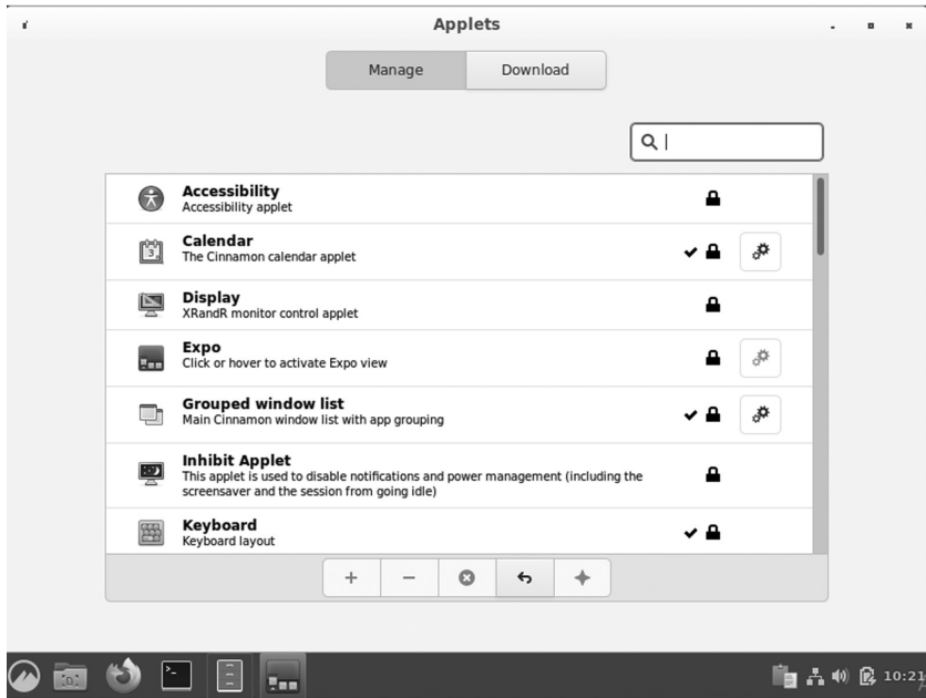
Applets.
