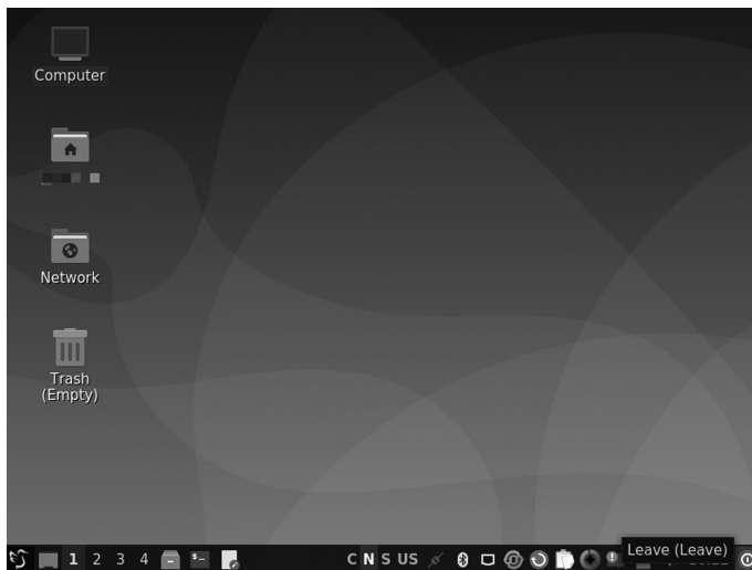
LXQt Desktop.
