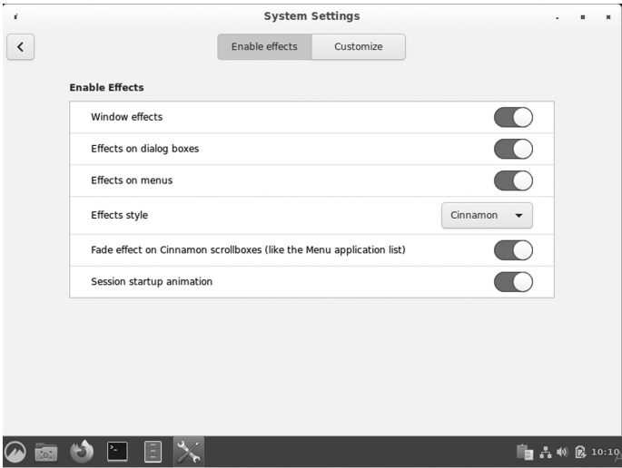
Effects Setting.
