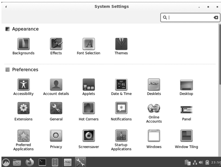
System Settings.
