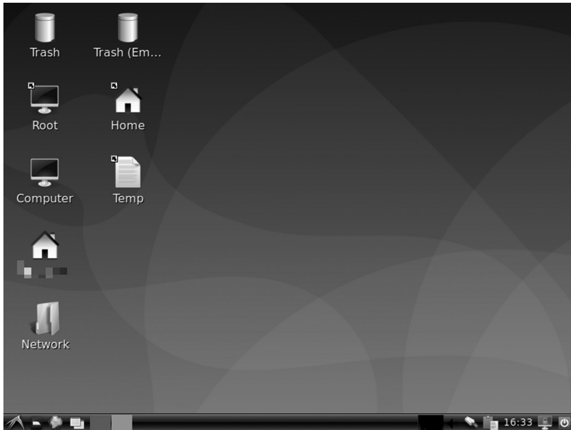
LXDE Desktop.
