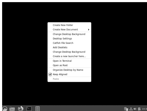
Customize Settings.
