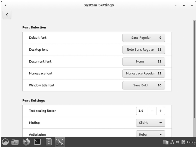
Font Selection.
