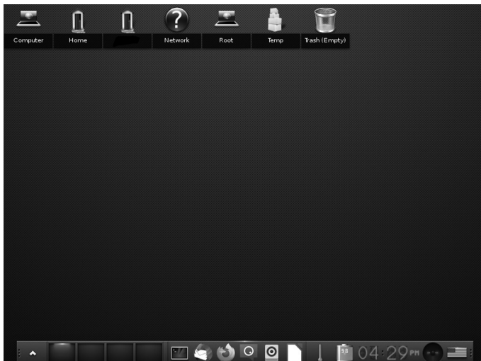
Enlightenment Desktop.
