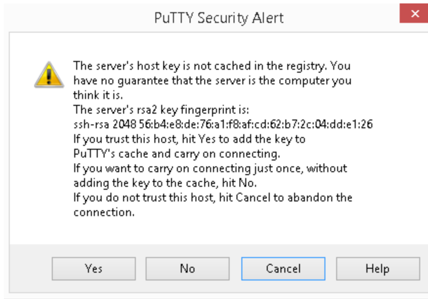
Figure 1-2. PuTTY alert
