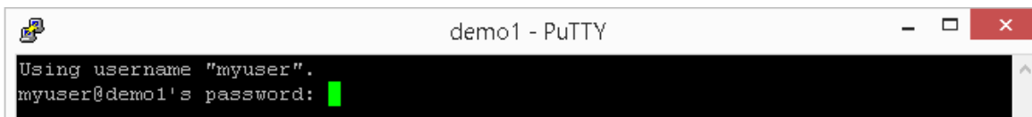
Figure 1-3. PuTTY password
