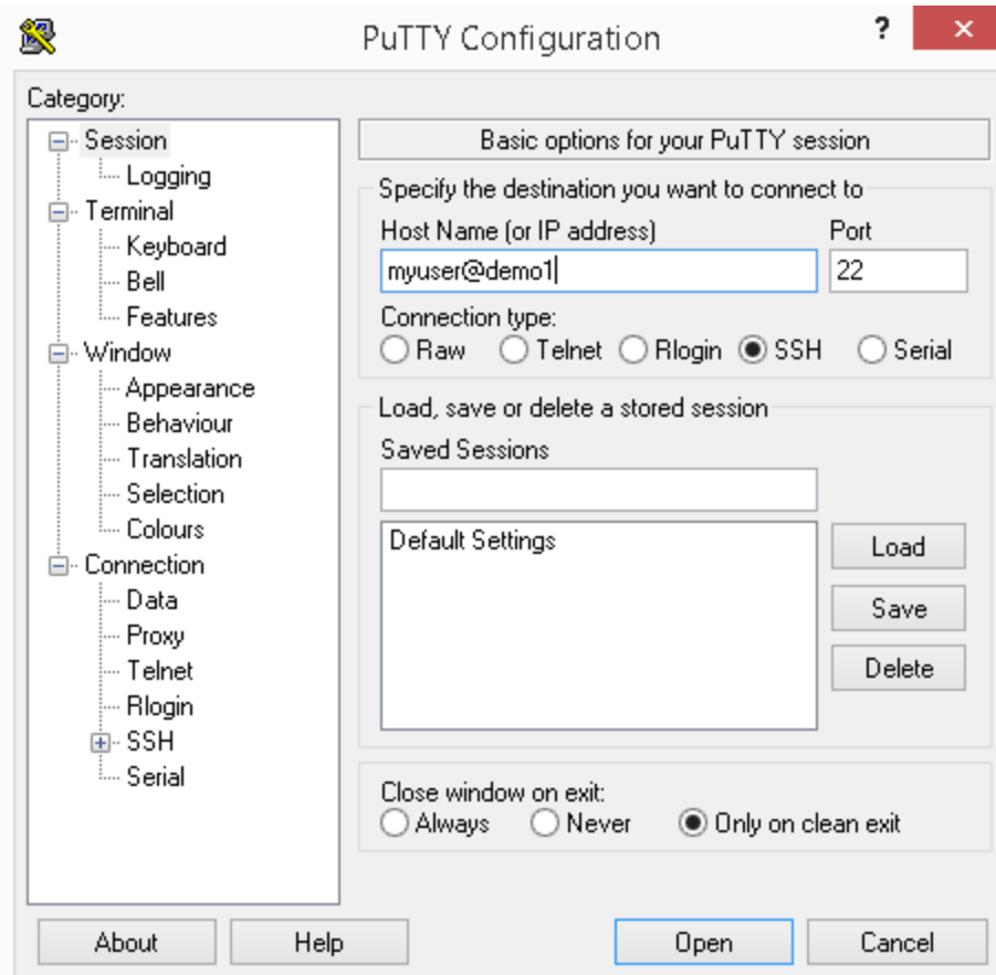
Figure 1-1. PuTTY prompt
